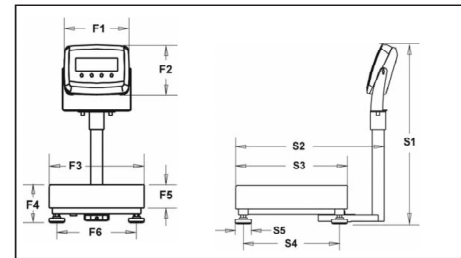
Outline Dimensions
